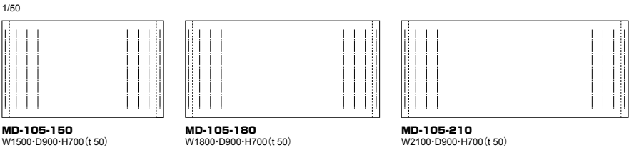
MD-105-150 W1500・D900・H700 (t 50) MD-105-180 W1800・D900・H700 (t 50) MD-105-210 W2100・D900・H700 (t 50)
