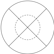
AD-033HL 150C: φ1500・H700(t 30)
