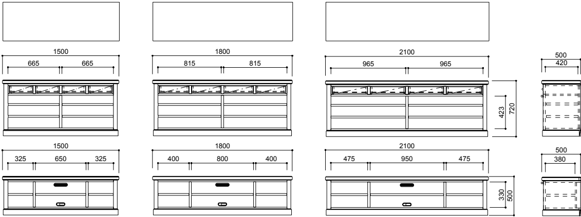
NC-048TV-150 W1500 × D500 × H500 NC-048SB-150 W1500 × D500 × H720 NC-048TV-180 W1800 × D500 × H500 NC-048SB-180 W1800 × D500 × H720 NC-048TV-210 W2100 × D500 × H500 NC-048SB-210 W2100 × D500 × H720
