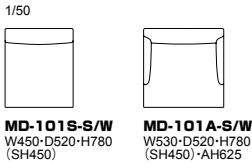
MD-101S-S/W W450・D520・H780 (SH450) MD-101A-S/W W530・D520・H780 (SH450)・AH625
