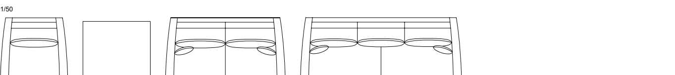
NC-030-1P W900 × D950 × H900 (SH400) AH580 NC-030-OT W900 × D900 (SH400) NC-030-2P W1600 × D950 × H900 (SH400) AH580 (Sクッション×2) NC-030-3P W2150 × D950 × H900 (SH400) AH580 (Sクッション×2)
