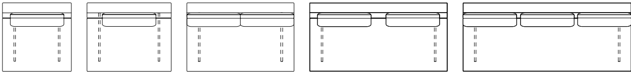
MD-1105-S-90 W900-D900-H760 (SH380) MD-1105-S-110 W1100-D900-H760 (SH380) MD-1105-S-140 W1400-D900-H760 (SH380) MD-1105-S-180 W1800-D900-H760 (SH380) MD-1105-S-220 W2200-D900-H760 (SH380)
