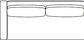
MD-805-3PR/3PL W1935・D900・H750 (SH380) AH530 (図面はMD-805-3PR右肘)
