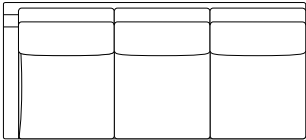
MD-505-3PR/3PL-H W2000・D900・H960 (SH400)・AH600 (図はMD-505-3PR-H右肘)
