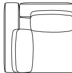
MD-805-CRR/CRL W900・D900・H750 (SH380) AH530 (図面はMD-805-CRR)
