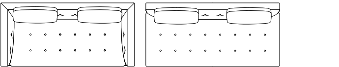
MD-705-2P W1800・D850・H850 (SH400)・AH720
