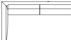
MD-210A-2PR/2PL W1500・D825・H770 (SH400) AH650 (図はMD-210A-2PR右肘)
