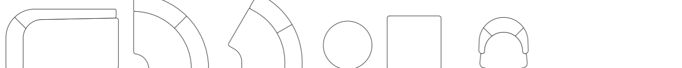
MD-3211-CLL/CLR W800-D1500-H710(SH400) MD-3211-C90 W1000-D1000-H710(SH400) MD-3211-C120 W987-D1016-H710(SH400) MD-3211-OT φ650-H400 MD-3211-OTS W720-D720-H400 MD-3211-1P W660-D700-H710(SH400)
