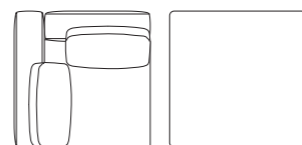
MD-805-CRR/CRL W900・D900・H750 (SH380) AH530 (図面はMD-805-CRR)
