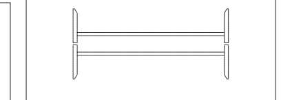
AD-887(240) W2400-D1200-H720(t 40)
