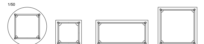
1/50 TA-007H-90C-W φ890-H550 TA-007H-60S-W W590-D590-H550 TA-007L-120-W W1190-D590-H350 TA-007L-90S-W W890-D890-H350
