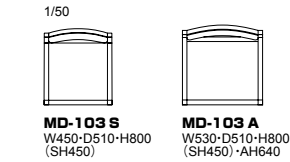
MD-103S W450・D510・H800 (SH450) MD-103A W530・D510・H800 (SH450)・AH640
