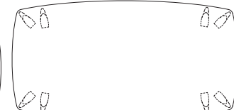
AD-115B(210) W2100-D1100-H700(t40)
