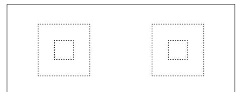
NC-029A-300 W3000 × D1200 × H720(t60)
