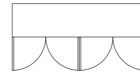
CA-002 Type-B W2100-D500-H640(W-H660) (図はアルミ脚)
