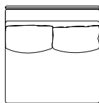
AD-085A-1P W900-D930-H750-SH400
